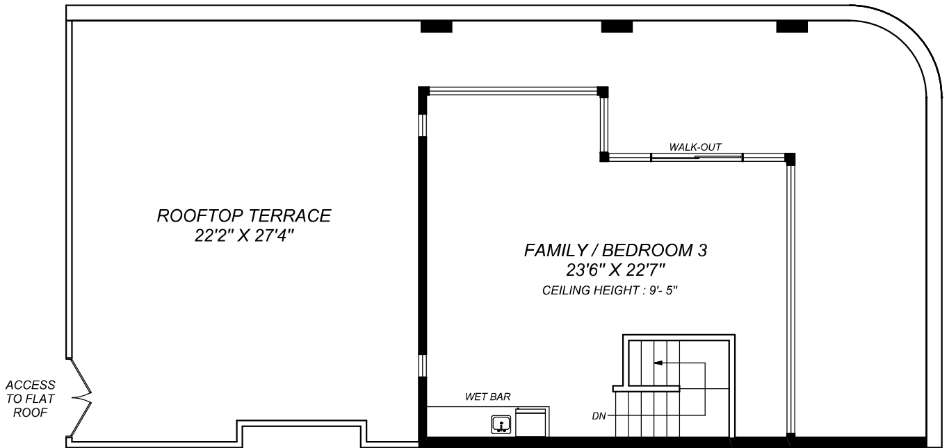
UPPER LEVEL 532 SQUARE FEET + TERRACE 983 SQUARE FEET
